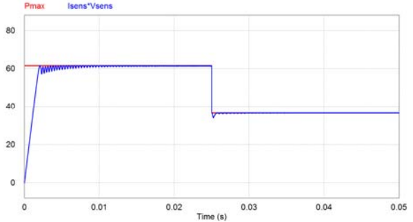
(b) Proposed INC in irradiation 1000w/m 2 → 200 w/m 2
