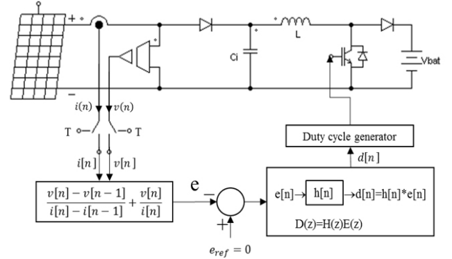
Fig.2 Proposed INC method
