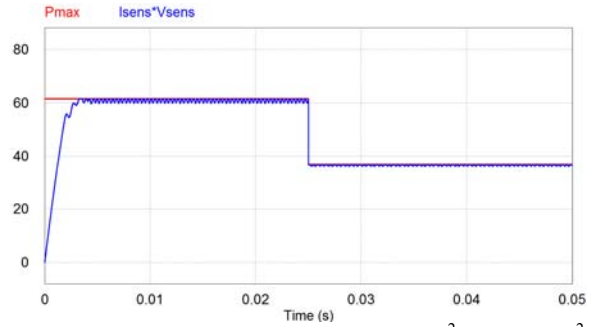
(a) Conventional INC in irradiation 1000w/m 2 → 200 w/m 2
