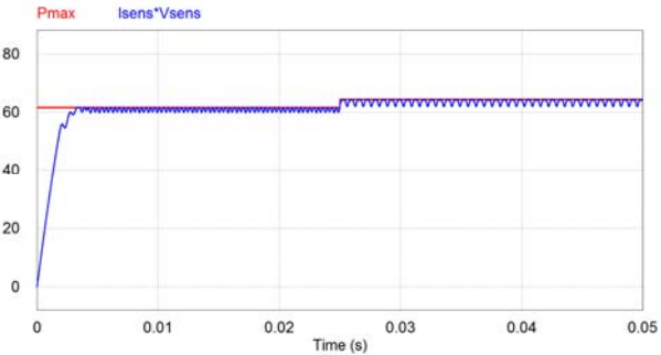
(c) Conventional INC in temperature 25 °C → 15 °C
