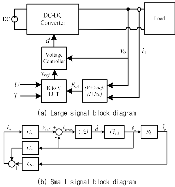
Fig. 8. Block diagrams.
