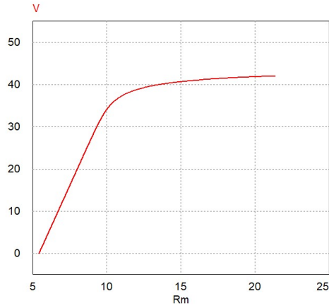
Fig. 7. Proposed Rm to V reference curve.
