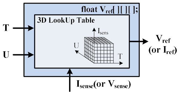
Fig. 2. Look-up table based solar array simulator engine.
