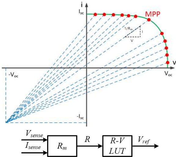
(c) Proposed impedance control with operating point projection
