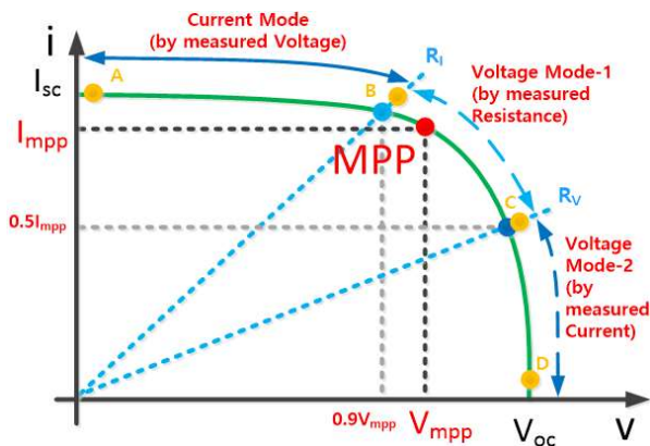
Fig. 4. Three-section hybrid control.
