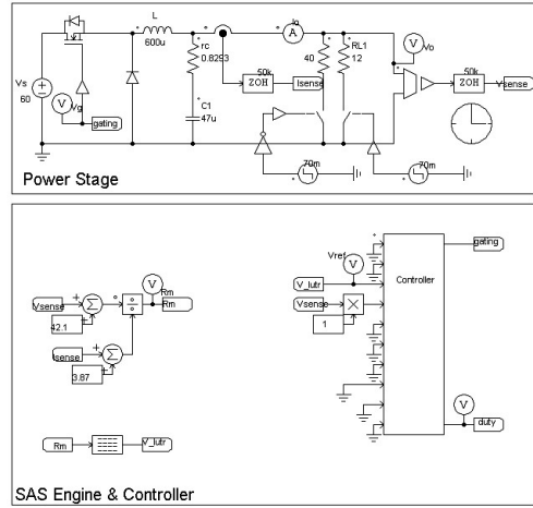
Fig. 9. Solar array simulator using PSIM.
