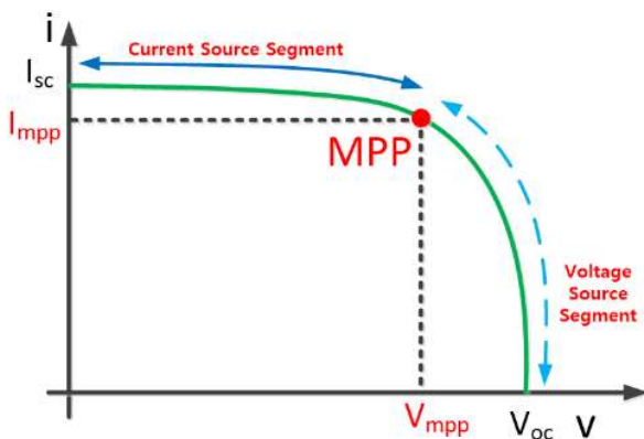
Fig. 3. Photovoltaic I-V characteristic curve.
