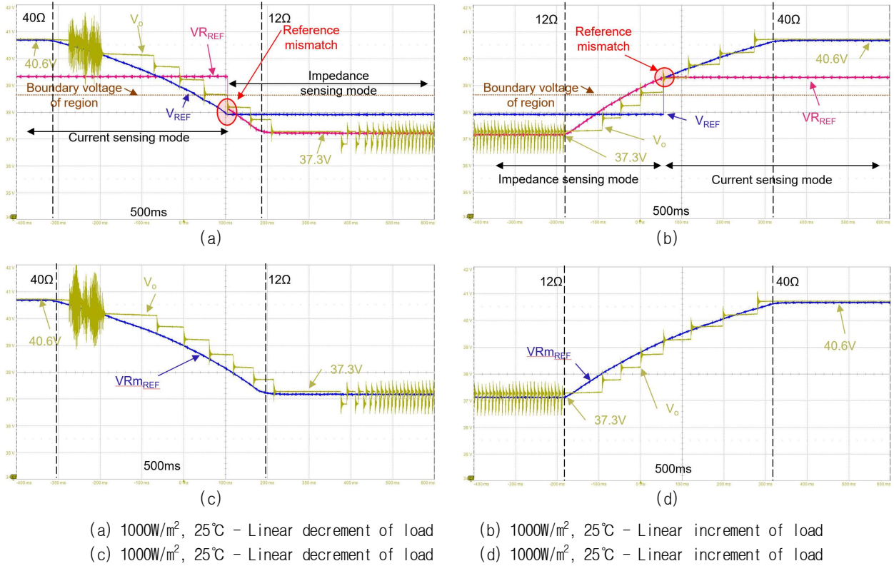
Fig. 14. Experiment result (Sequence mode): (a)-(b) Conventional method, (c)-(d) Proposed method.
