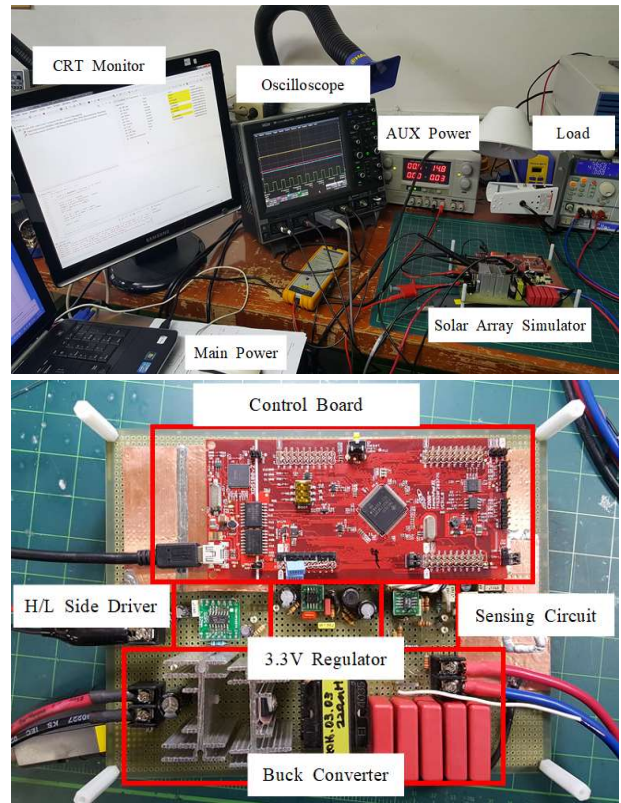
Fig. 13. Experimental setup.
