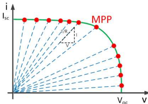
(a) Conventional current/voltage mode control
